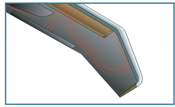
Flaw Tolerant Blades, Rotor Ice Protection System and Integrated Tip Cap
